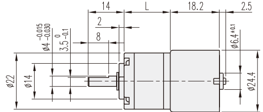
GEARHEAD LENGTH
