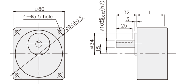
GEAR HEAD K8G□B(C)
