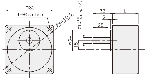
GEARHEAD K8G□B(C)
