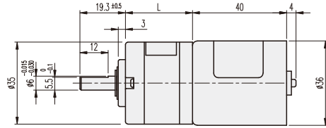
GEARHEAD LENGTH
